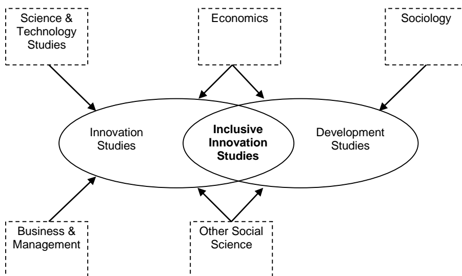
Figure 3: Disciplinary Foundations for Inclusive Innovation Research
